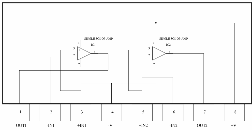
DUAL OP-AMP SIL PACKAGE
