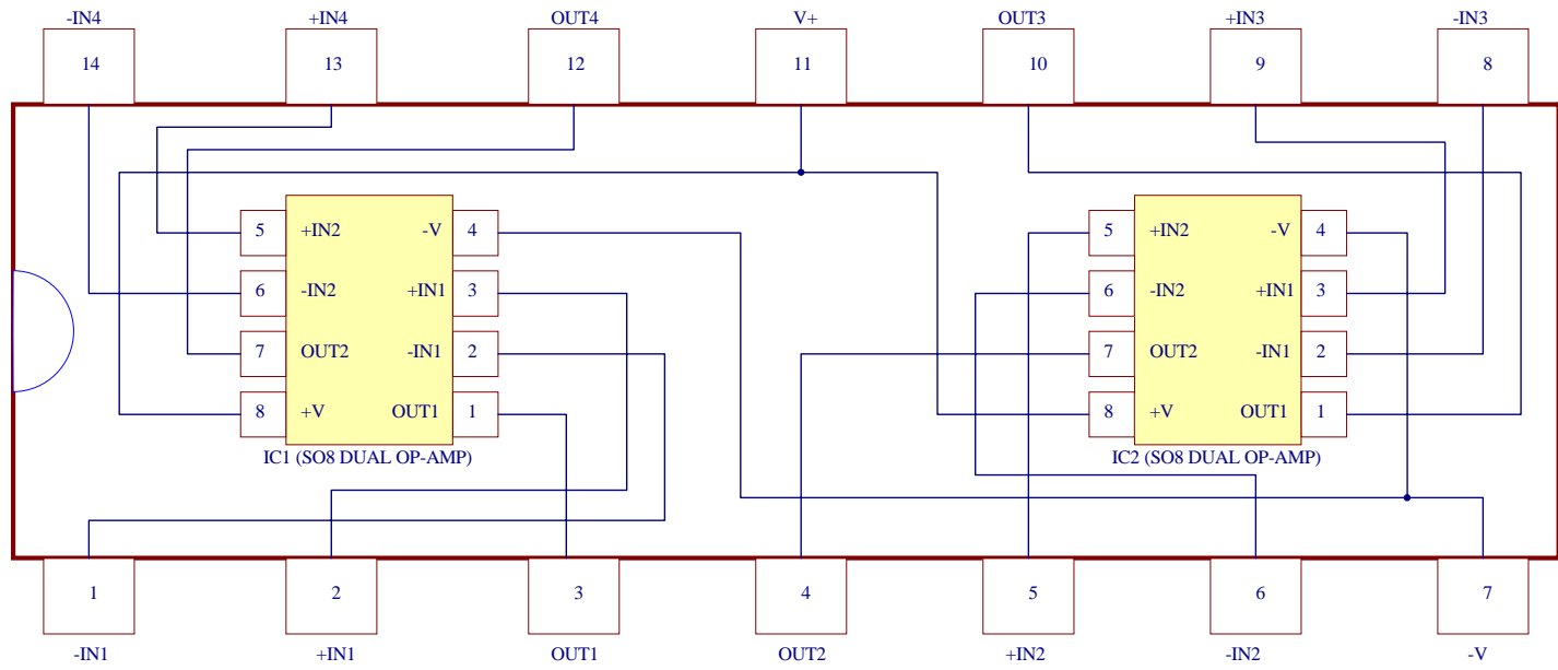
QUAD OP-AMP DIP PACKAGE (RC4136 PINOUT)
