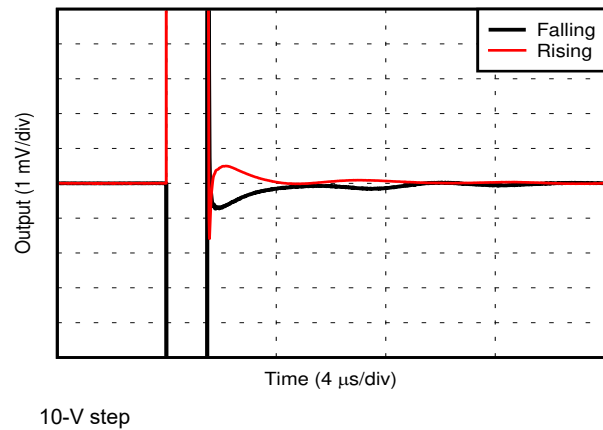
Figure 6-38. Settling Time
