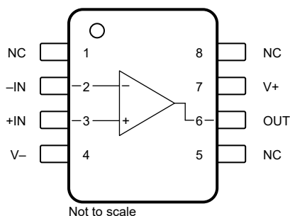
Figure 5-1. OPA210: D (8-Pin SOIC) and DGK (8-Pin VSSOP, Preview) Packages, Top View
