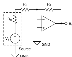
(B) Noise in Inverting Gain Configuration
