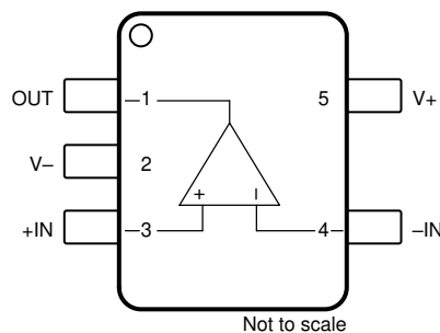
Figure 5-2. OPA210: DBV (5-Pin SOT-23, Preview) Package, Top View
