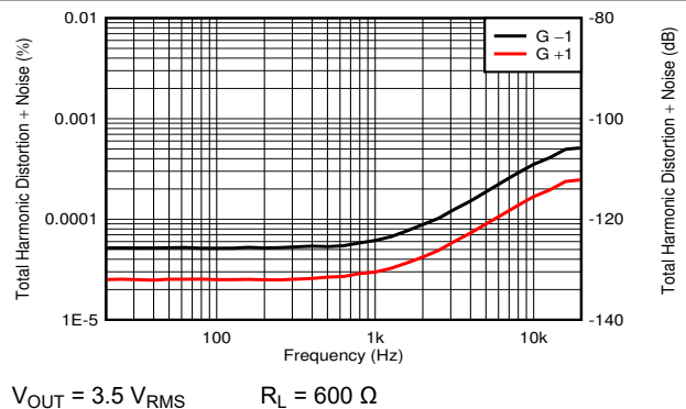
Figure 6-6. THD+N Ratio vs Frequency
