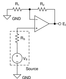
(A) Noise in Noninverting Gain Configuration
