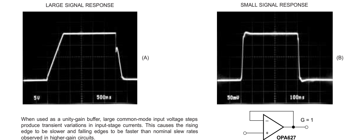
Figure 40. OPA627 Dynamic Performance, G = 1
